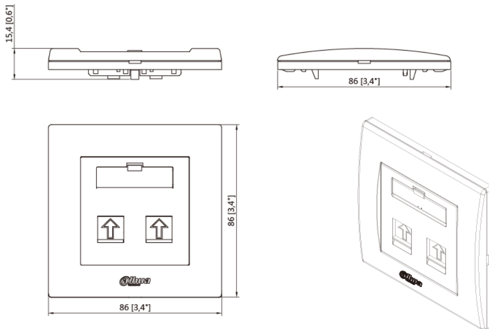
DH-PFM971-2_dimension
